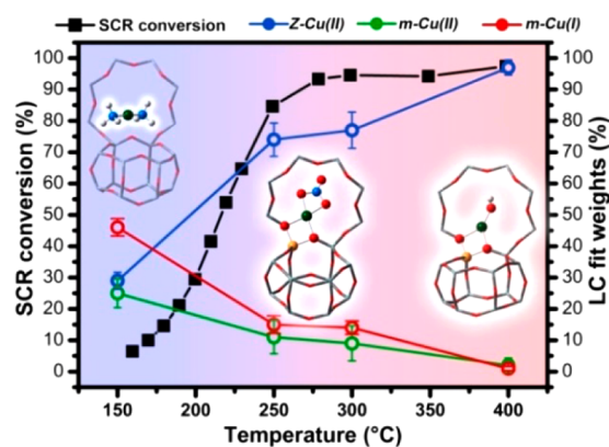
Figure 4. Comparison between temperature-dependent NH 3 SCR conversion rate and Cu-speciation in Cu-CHA. Structural snapshots of the dominant (highest relative abundance over the total number of Cu sites) model Cu-species evidenced by LCF analysis of operando XANES for each probed temperature are also reported, including Z-[Cu(II)OH - ] and Z-[Cu(II)NO 3 - ] in the high-temperature range and mobile Cu(I) (NH 3 ) 2 complexes in the low-temperature range (atoms color code: Cu: green, O: red, Al: yellow, Si: gray, N: blue, H: white).
