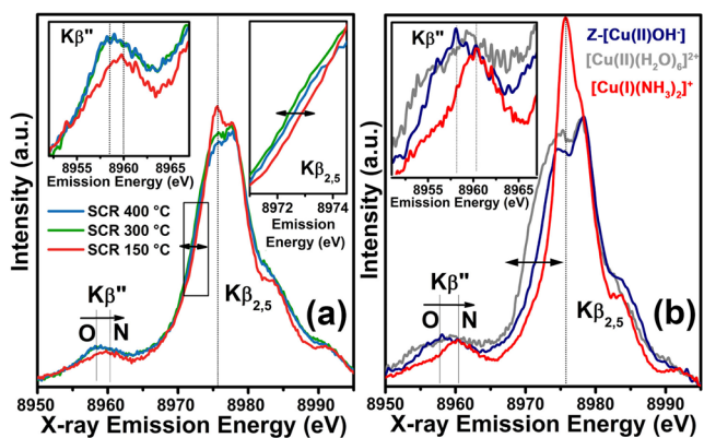
Figure 3. (a) Background-subtracted operando XES spectra collected during SCR at temperatures of 150, 300, 400 °C. (b) Background-subtracted XES spectra of selected Cu reference states formed inside the pores of Cu-CHA, representative of Z-Cu(II), m-Cu(II) and m-Cu(I) species. The insets report magnifications of the K\beta'' satellites and, for part (a) only, of the left side of the K\beta_{2,5} line, highlighted by the black boxes in the main panels.
